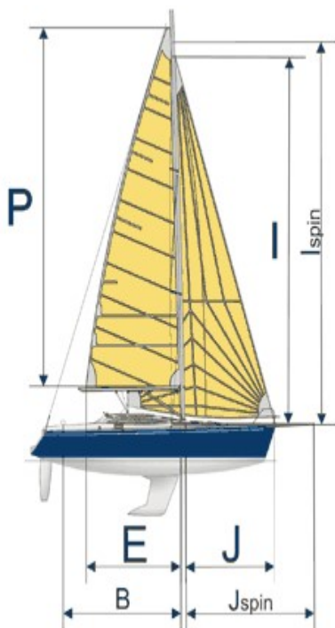
Rig Measurements
